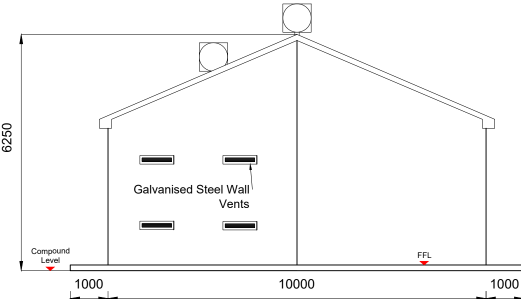
Elevation C Scale 1:100
